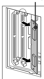
2. Remove Memory SIMM
